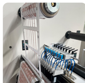
Auto Waste Remove + Counting Function+ Slitting Cutting
